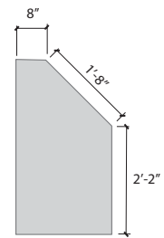
Section View
