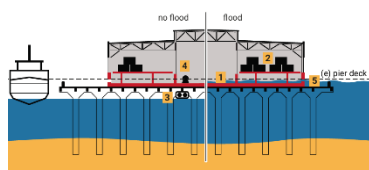
Wet Floodproofing
