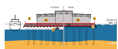
Structure Elevation
