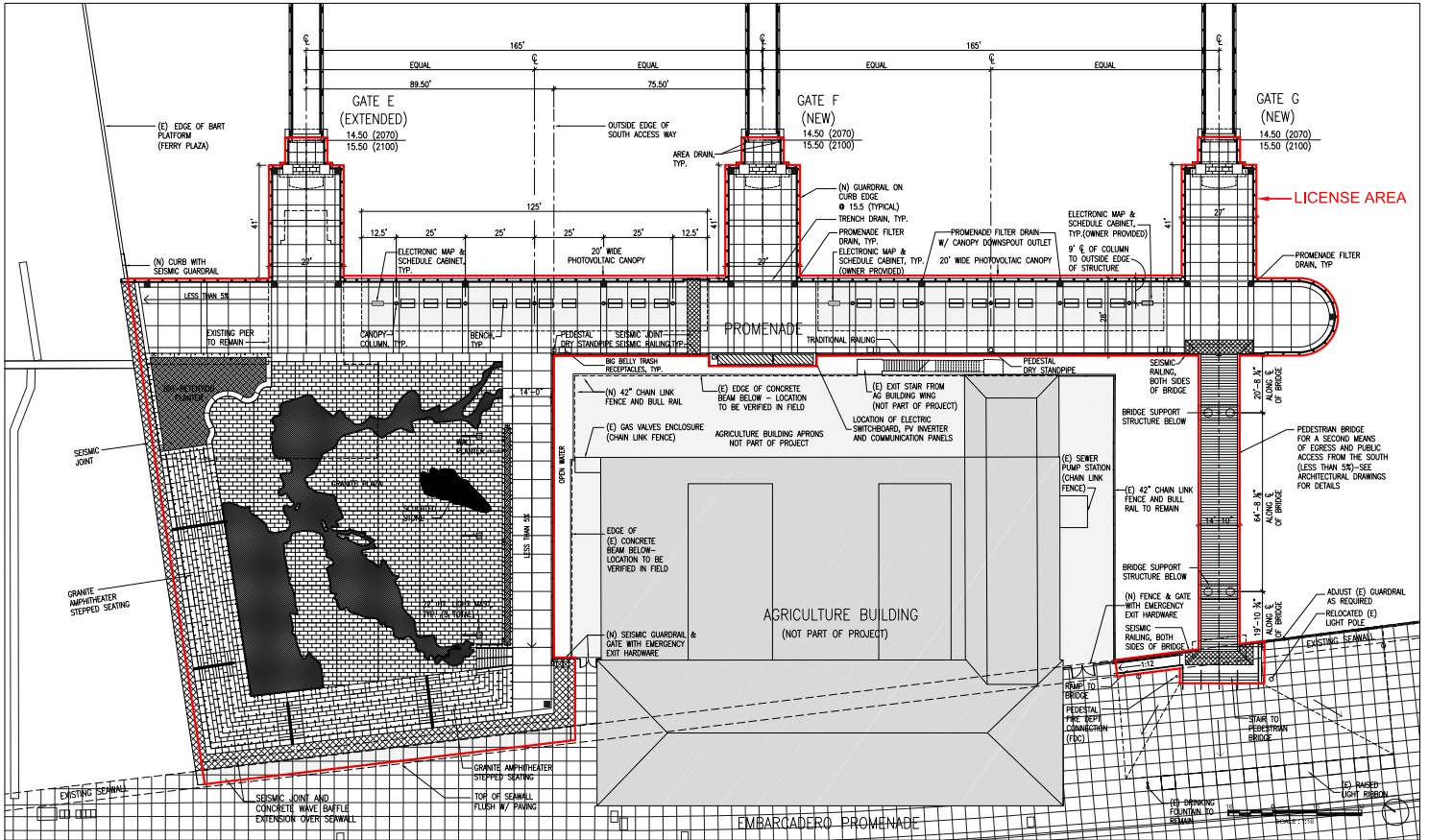
LICENSE AREA DIAGRAM
