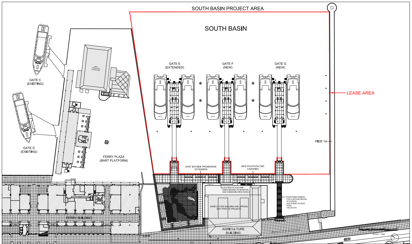
LEASE AREA DIAGRAM
